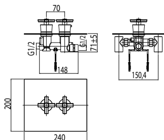
codice/code NCX27200 cartuccia/cartridge 00622444 vitone/valve 00622430
