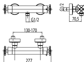
codice/code NCX26200 cartuccia/cartridge 00621435 vitone/valve 00622424
