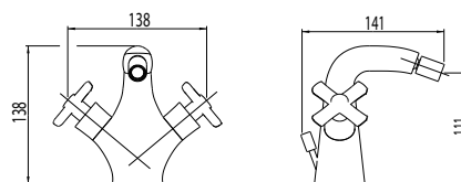
codice/code NCX02200 vitone/valve 00622424
