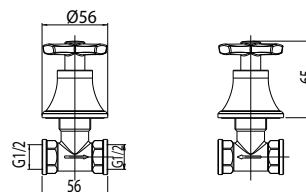
codice/code NCX01700 vitone/valve 00622424
