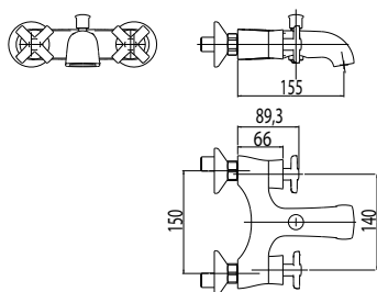
codice/code NCX00500 vitone/valve 00622430
