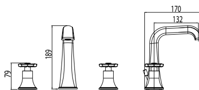
codice/code NCX00400 vitone/valve 00622429
